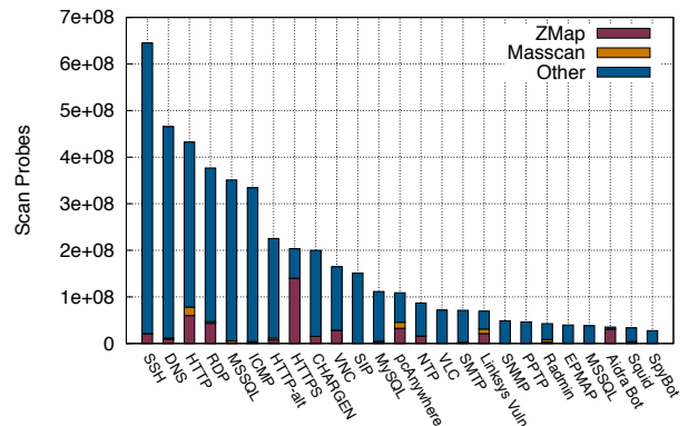
Figure 3: Large scans ( \geq 10\% ) by software — We fingerprint ZMap and Masscan probes and present the breakdown of large scans that use these scanners.
