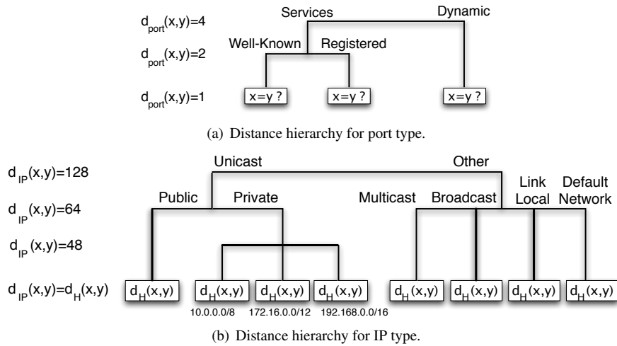
Figure 1. Distance metrics for categorical types of port and IP. Distances listed to the left indicate the distance when values diverge at that level of the hierarchy.
