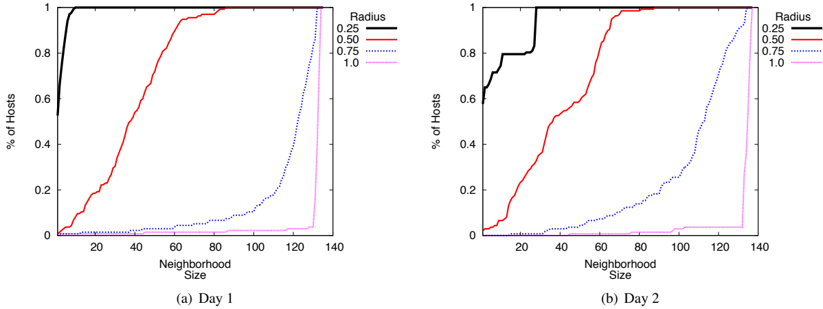
Figure 6. Privacy neighborhood sizes for different distance radius settings.
