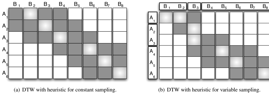
Figure 3. Example dynamic programming matrices with the original Sakoe-Chiba heuristic (a) and our adapted heuristic (b) for variable sampling rate time series. Gradient cells indicate the “diagonals” and dark shaded cells indicate the window around the diagonal that are evaluated. In the the variable rate example, points in the same subsequence are grouped together.
