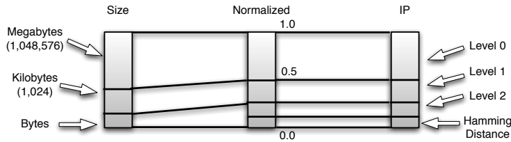
Figure 2. Example piecewise normalization of size and IP types. Mapping each range independently ensures they are weighted in accordance with the relative severity of the distance.
