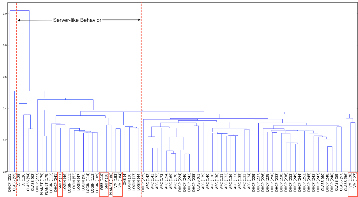
Figure 4. Dendrogram illustrating agglomerative clustering using DTW-based metric on hosts in the first day of the CSE dataset.
